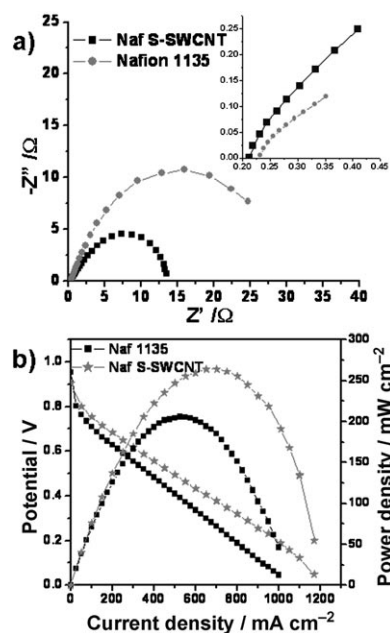
Figure 3. a) Nyquist impedance ( Z ) plots for MEAs made with Nafion 1135 and Nafion/S-SWCNT membranes. The measurements were carried out at room temperature with a flow of humidified \text{H}_2 and \text{O}_2 . Inset: the high-frequency range at higher magnification. b) Polarization curves obtained with Nafion/S-SWCNT and Nafion 1135 membranes at 60^{\circ}\text{C} with humidified \text{H}_2 and \text{O}_2 (flow rate 0.4 \text{ slpm} ). The cells were conditioned for 30 min at open-circuit potential and at 0.2 \text{ V} for 15 min before measurements.
